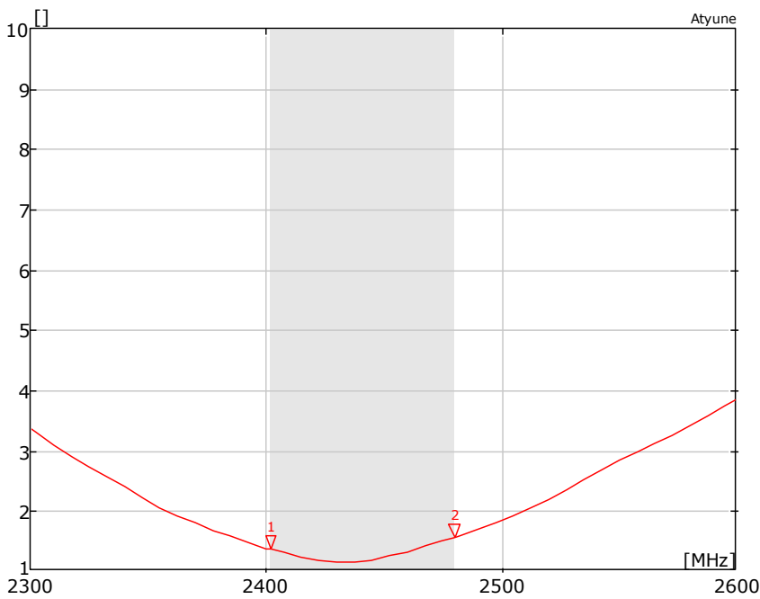
All data measured on Antenova's evaluation PCB Part No. SRCW004-EVB-1 (EVK size 60mm x 37mm)
